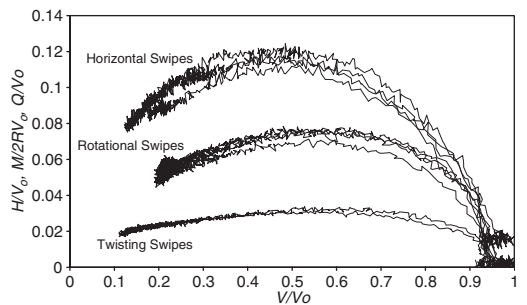
Figure 11. Results normalised by V_0 .
