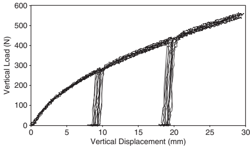
Figure 8. Typical vertical loading results.
