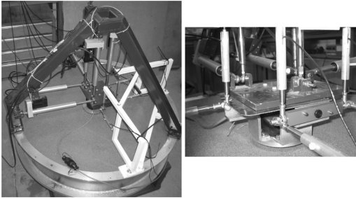
Figure 4. Photos of the 6dof loading rig including a close-up of the small LVDT measurement system.
