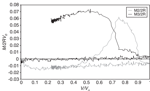
Figure 13. A swipe test where consecutive rotations are performed.
