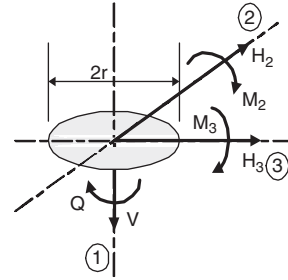
Figure 3. 6dof loading on a circular foundation.
