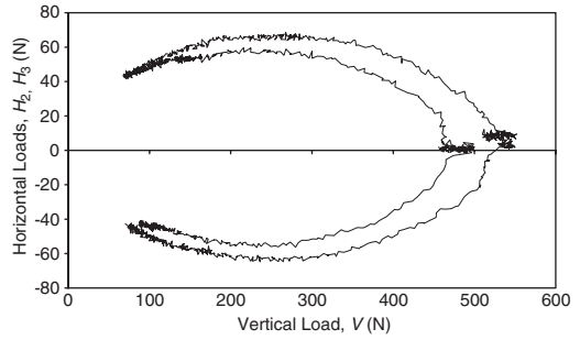
Figure 10. Horizontal swipe results.
