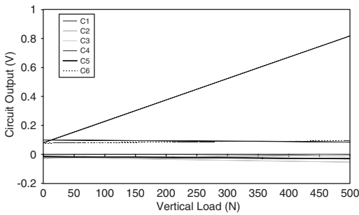
Figure 7. Calibration curves for the loadcell under vertical loading.
