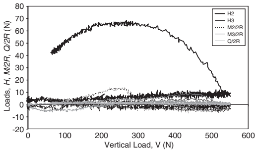
Figure 9. A horizontal swipe result.
