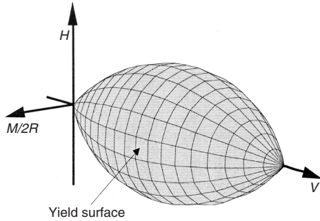
Figure 2. Yield surface for shallow foundations.
