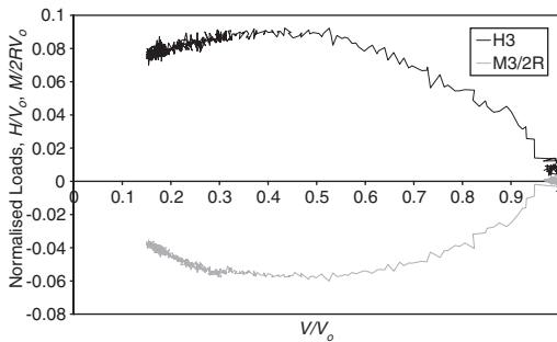
Figure 12. Non co-planar loading applied to the foundation.
