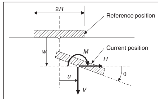
Figure 1. Sign conventions for 3 degree-of-freedom loading (Butterfield et al. 1997).
